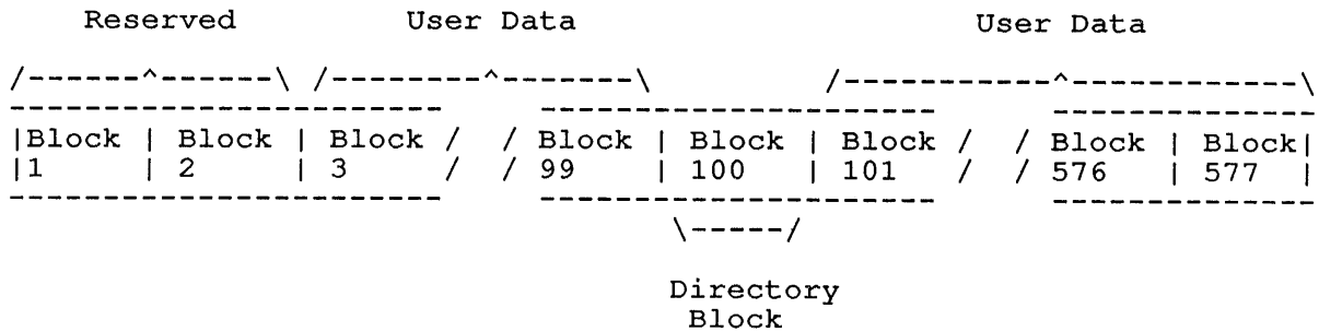
Figure 13-2: DECTape Format
