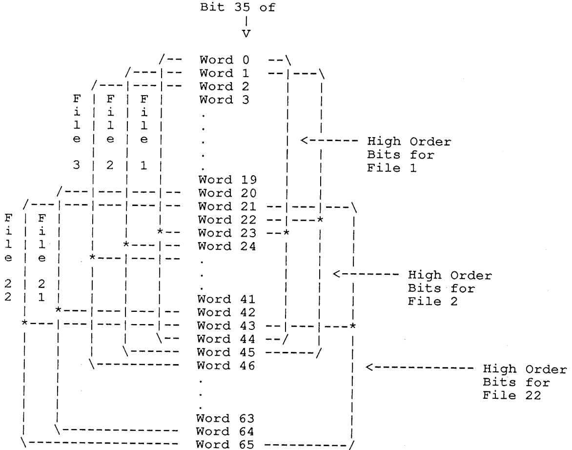
Figure 13-8: High-Order Three Bits of Creation Date
