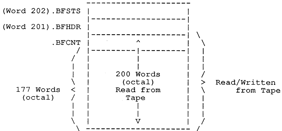
Figure 13-1: DECTape Buffer
