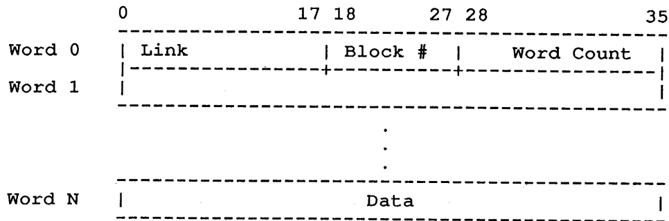
Figure 13-9: Data Block Format
