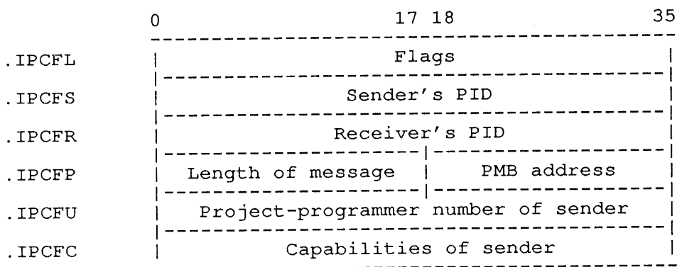
Figure 7-1: Packet Header Block
