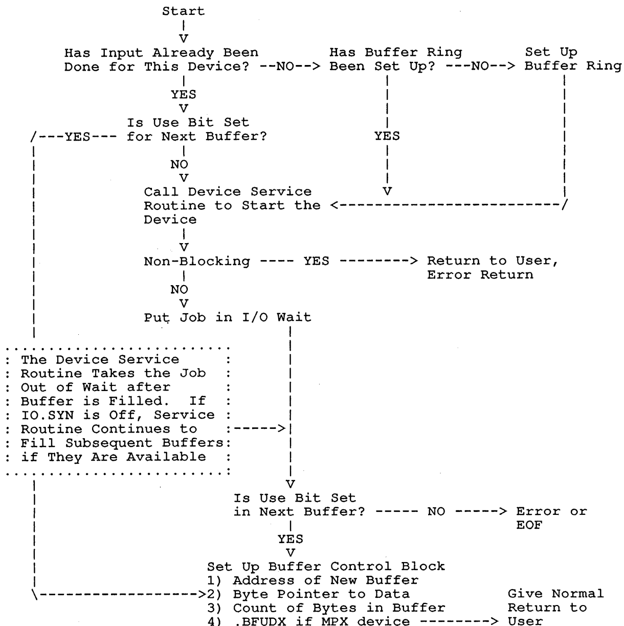
Figure 11-3: Flowchart for Buffered Input
