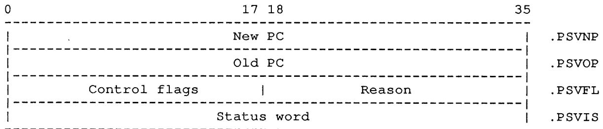
Figure 6-2: Interrupt Control Block
