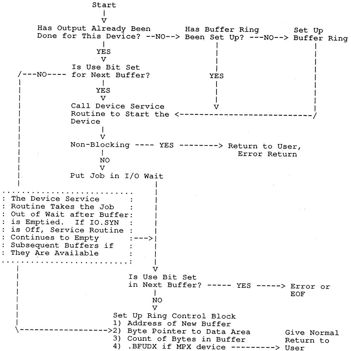
Figure 11-4: Flowchart for Buffered Output
