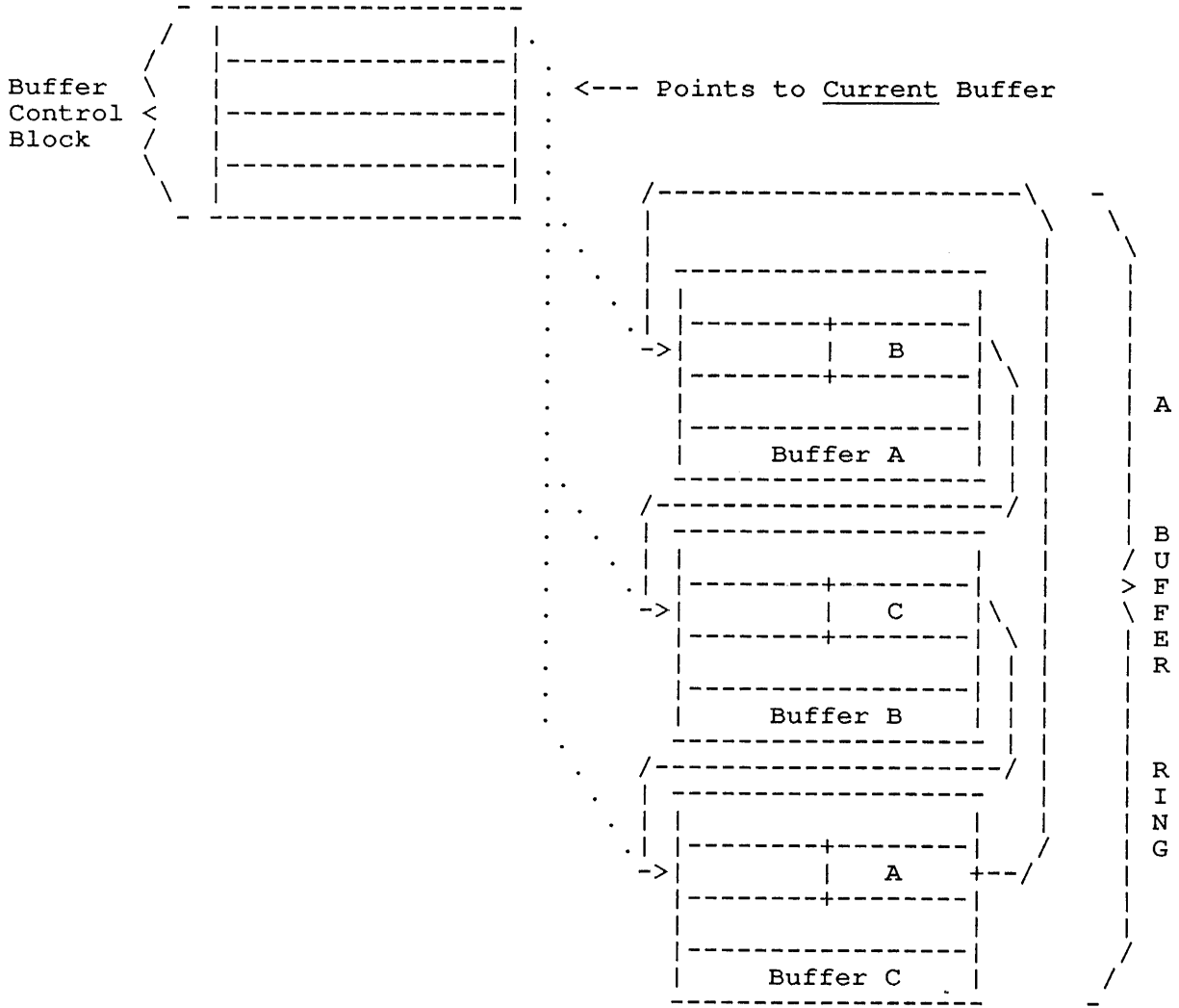
Figure 11-2: The Buffer Structure
