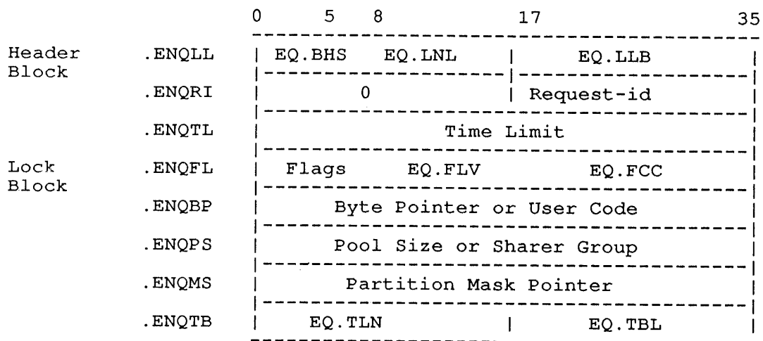
Figure 8-1: ENQ/DEQ Request Block
