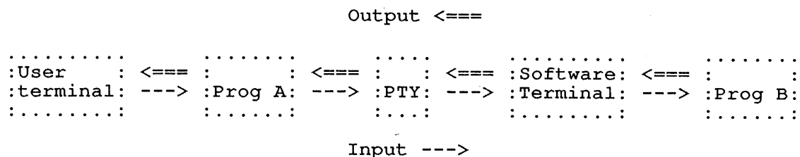
Figure 15-1: PTY I/O
