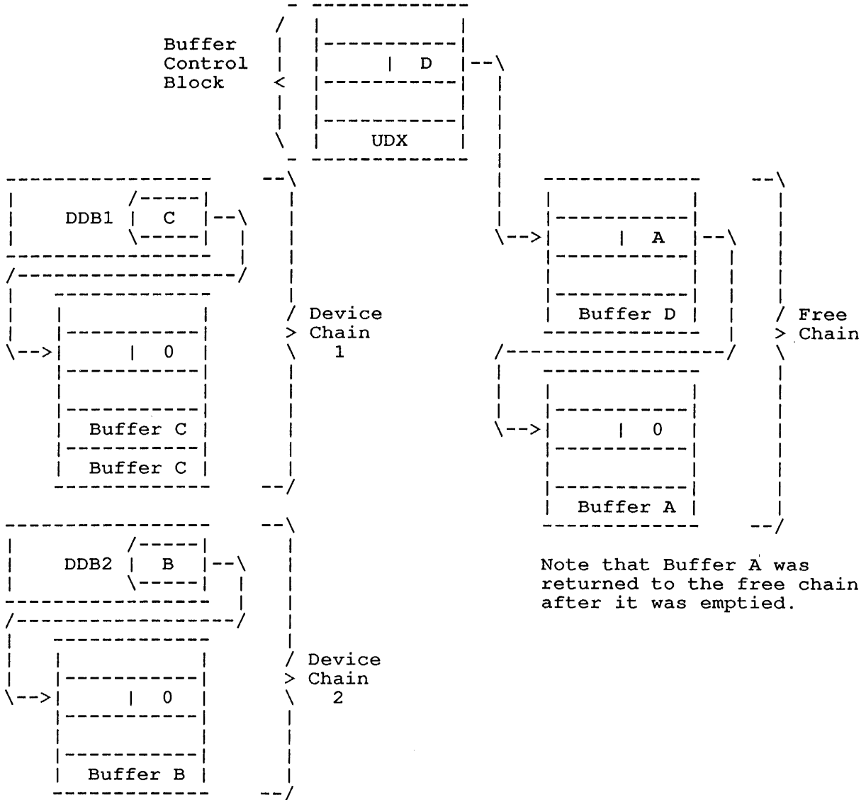
Figure 11-7: One Buffer Moved Back to Free Chain
